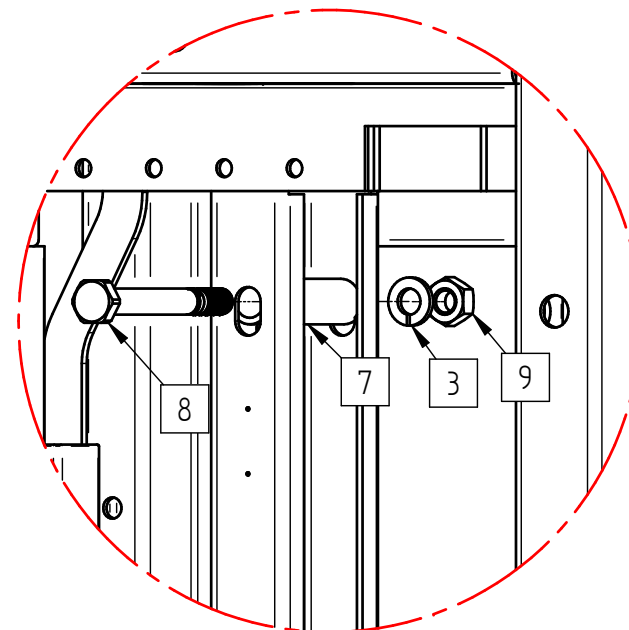
DETAIL C
